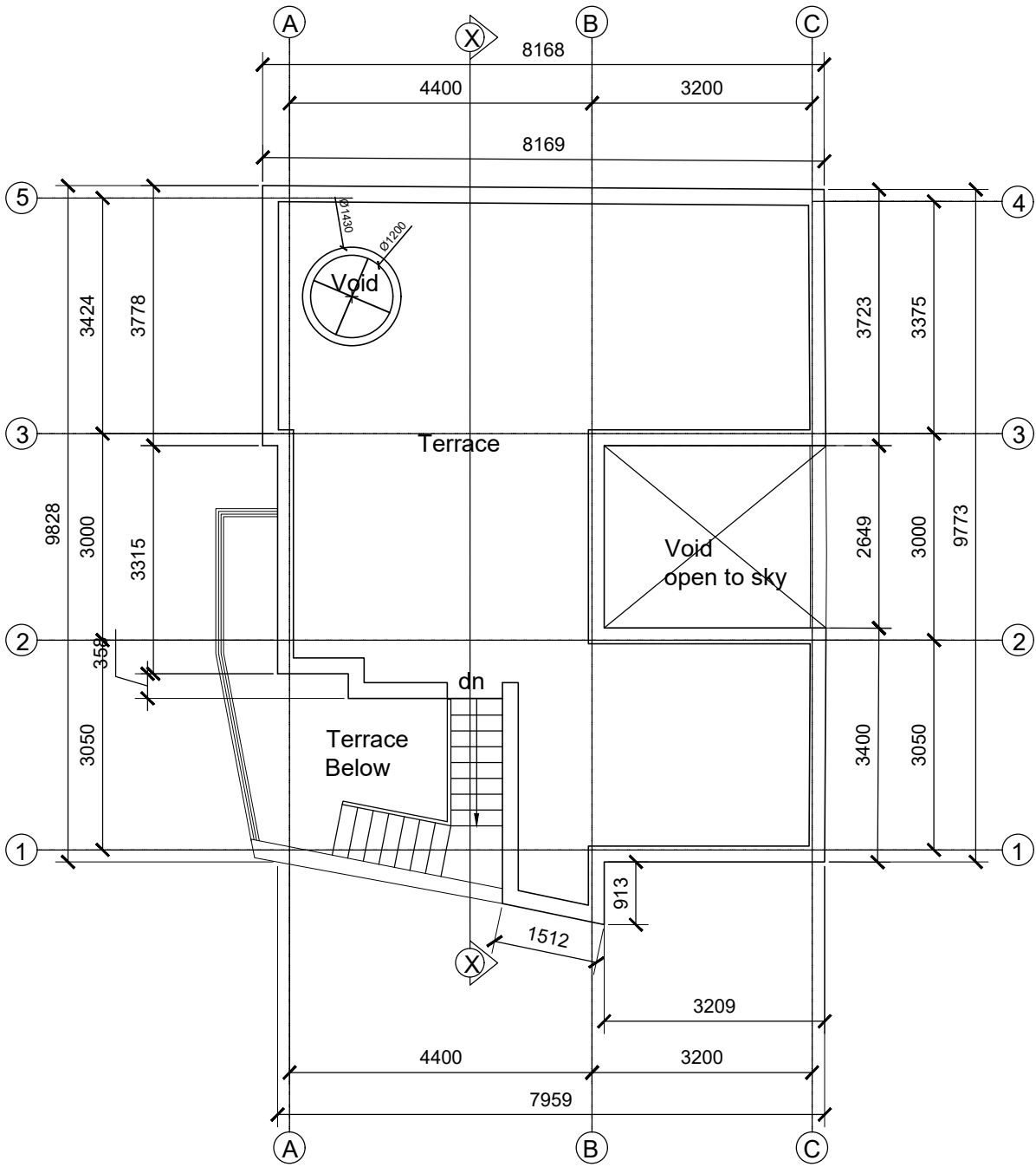
ROOF PLAN
